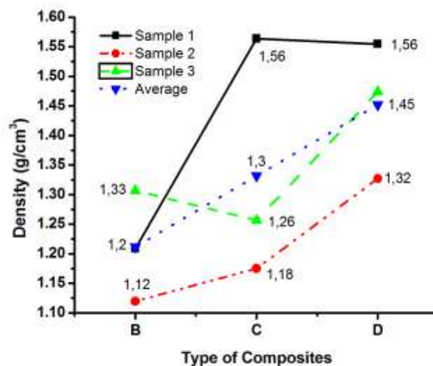
Figure 2. The Density of Hybrid Composites
