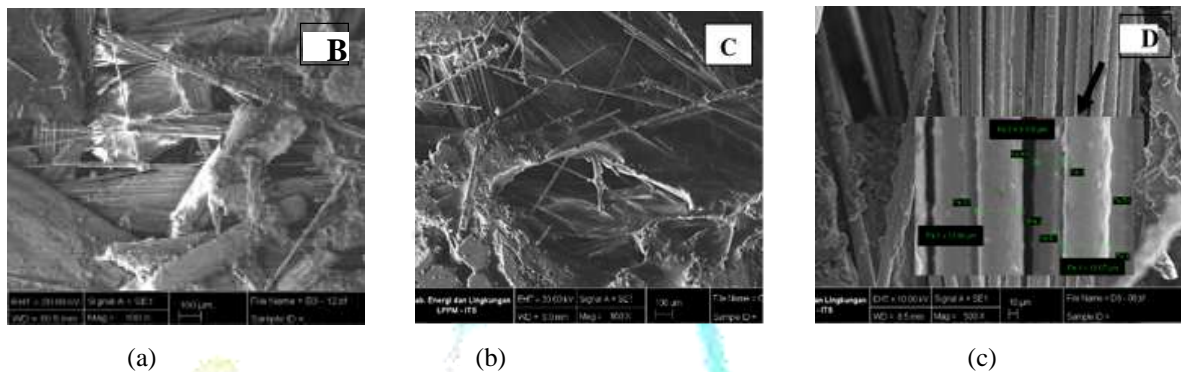
Figure 7. SEM Results of Hybrid Composites
