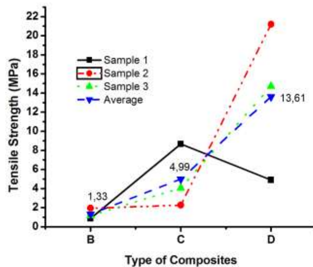
Figure 3. The Tensile Strength of Hybrid Composites
