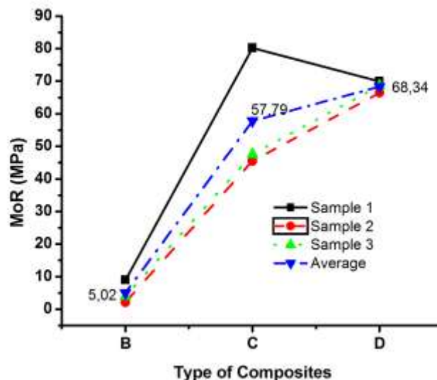
Figure 6. The MoR of Hybrid Composites
