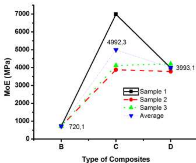
Figure 5. The MoE of Hybrid Composites
